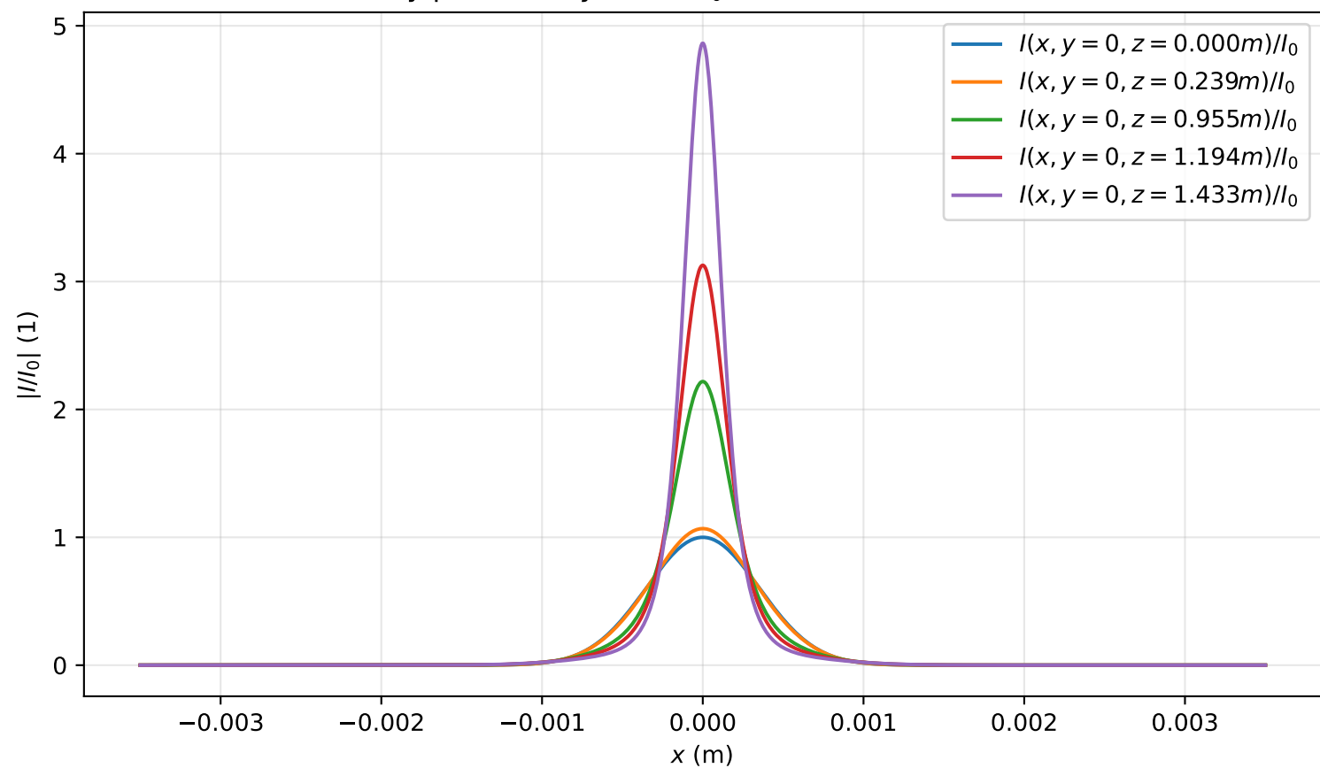
Intensity profile I(x, y = 0, z)/I_0 , P_{in}=1.4P_{cr} , artificial time
